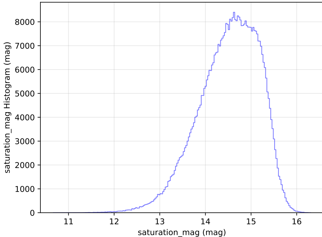
too_elab_heavy_r32_d3_gz_v3.4_10yrs All sky r band: saturation_mag Histogram
