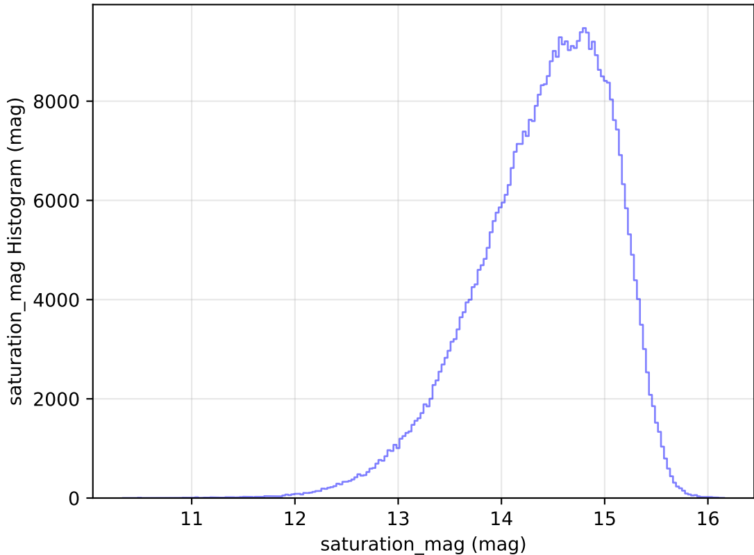
too_elab_heavy_r32_d3_gz_v3.4_10yrs All sky i band: saturation_mag Histogram
