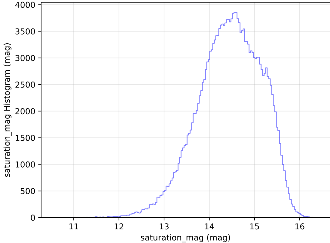
too_elab_heavy_r32_d3_gz_v3.4_10yrs All sky g band: saturation_mag Histogram
