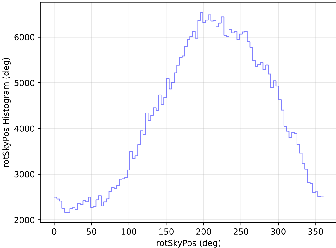
too_elab_heavy_r32_d3_gz_v3.4_10yrs WFD z band: rotSkyPos Histogram
