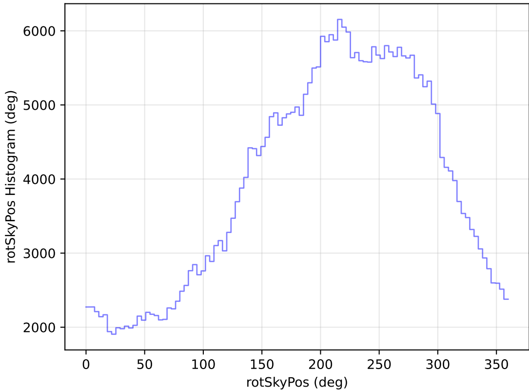
too_elab_heavy_r32_d3_gz_v3.4_10yrs WFD y band: rotSkyPos Histogram
