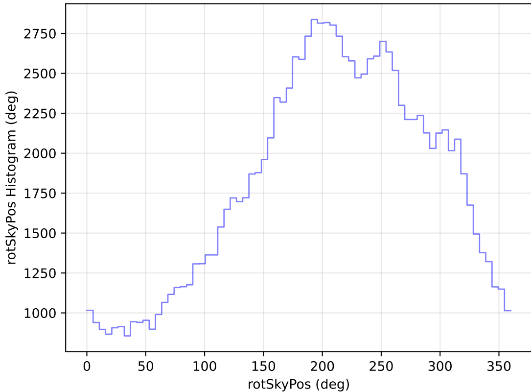
too_elab_heavy_r32_d3_gz_v3.4_10yrs WFD u band: rotSkyPos Histogram
