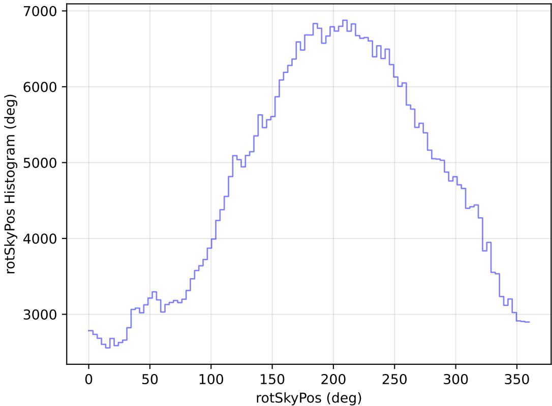
too_elab_heavy_r32_d3_gz_v3.4_10yrs WFD r band: rotSkyPos Histogram
