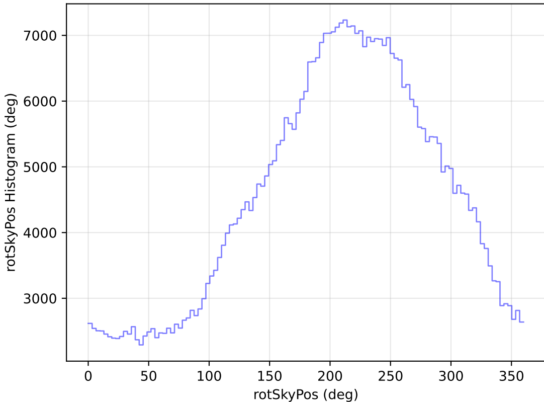
too_elab_heavy_r32_d3_gz_v3.4_10yrs WFD i band: rotSkyPos Histogram
