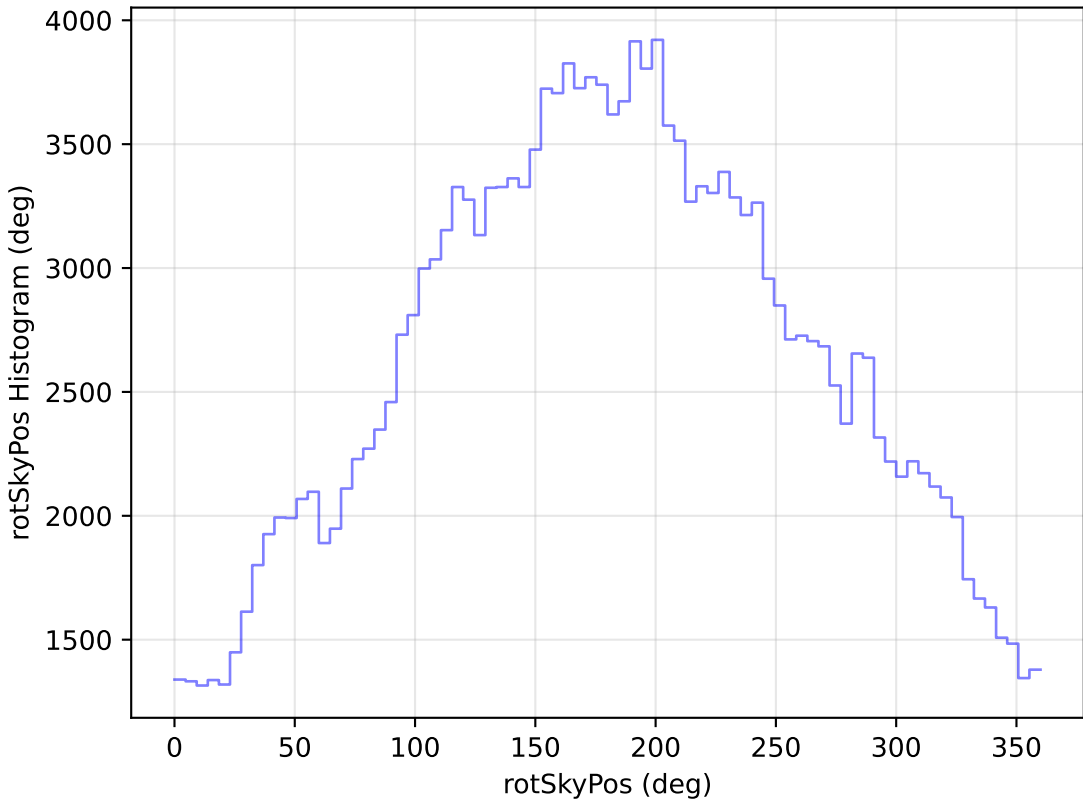
too_elab_heavy_r32_d3_gz_v3.4_10yrs WFD g band: rotSkyPos Histogram
