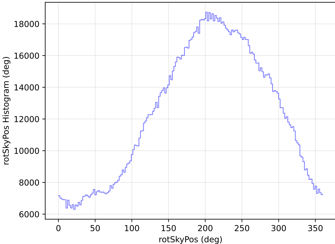
too_elab_heavy_r32_d3_gz_v3.4_10yrs WFD all bands: rotSkyPos Histogram
