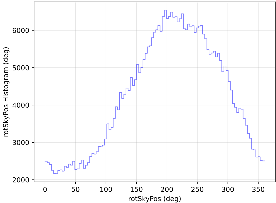
too_elab_heavy_r32_d3_gz_v3.4_10yrs All sky z band: rotSkyPos Histogram
