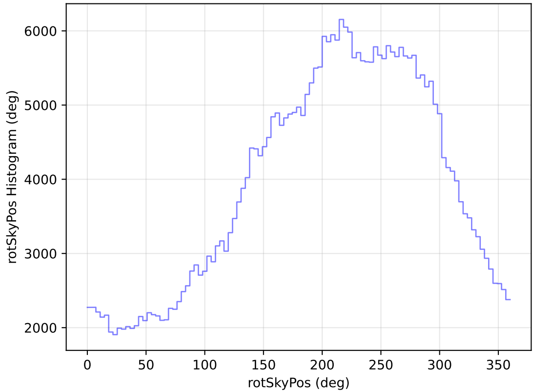
too_elab_heavy_r32_d3_gz_v3.4_10yrs All sky y band: rotSkyPos Histogram
