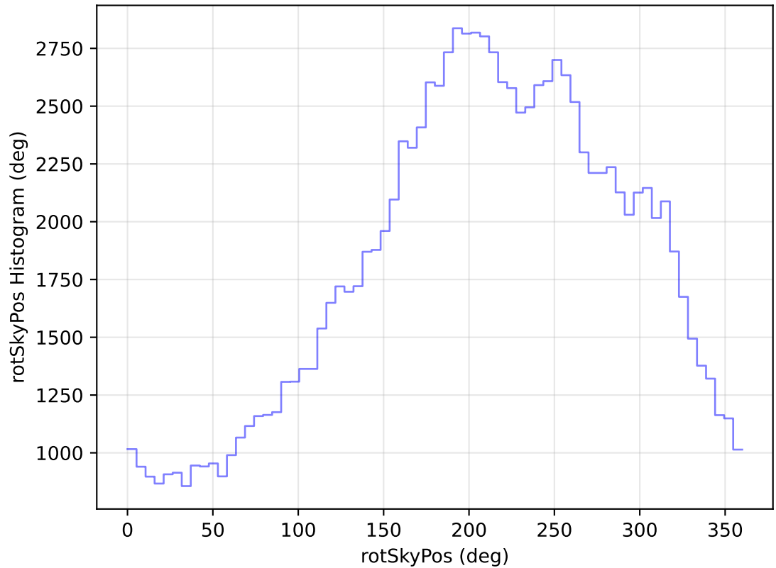
too_elab_heavy_r32_d3_gz_v3.4_10yrs All sky u band: rotSkyPos Histogram
