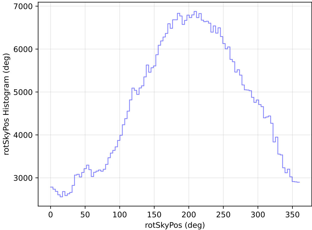
too_elab_heavy_r32_d3_gz_v3.4_10yrs All sky r band: rotSkyPos Histogram
