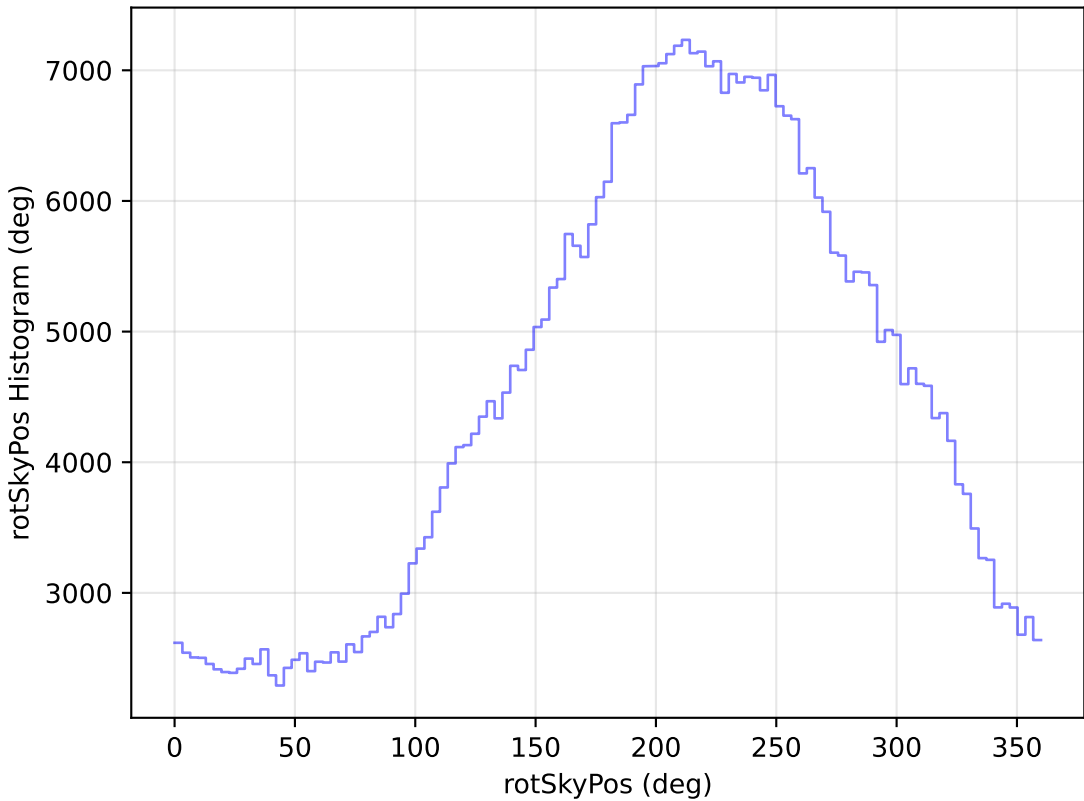
too_elab_heavy_r32_d3_gz_v3.4_10yrs All sky i band: rotSkyPos Histogram
