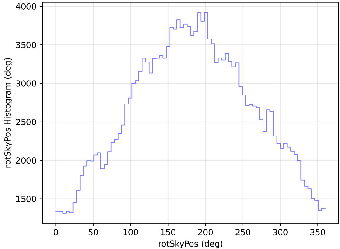
too_elab_heavy_r32_d3_gz_v3.4_10yrs All sky g band: rotSkyPos Histogram
