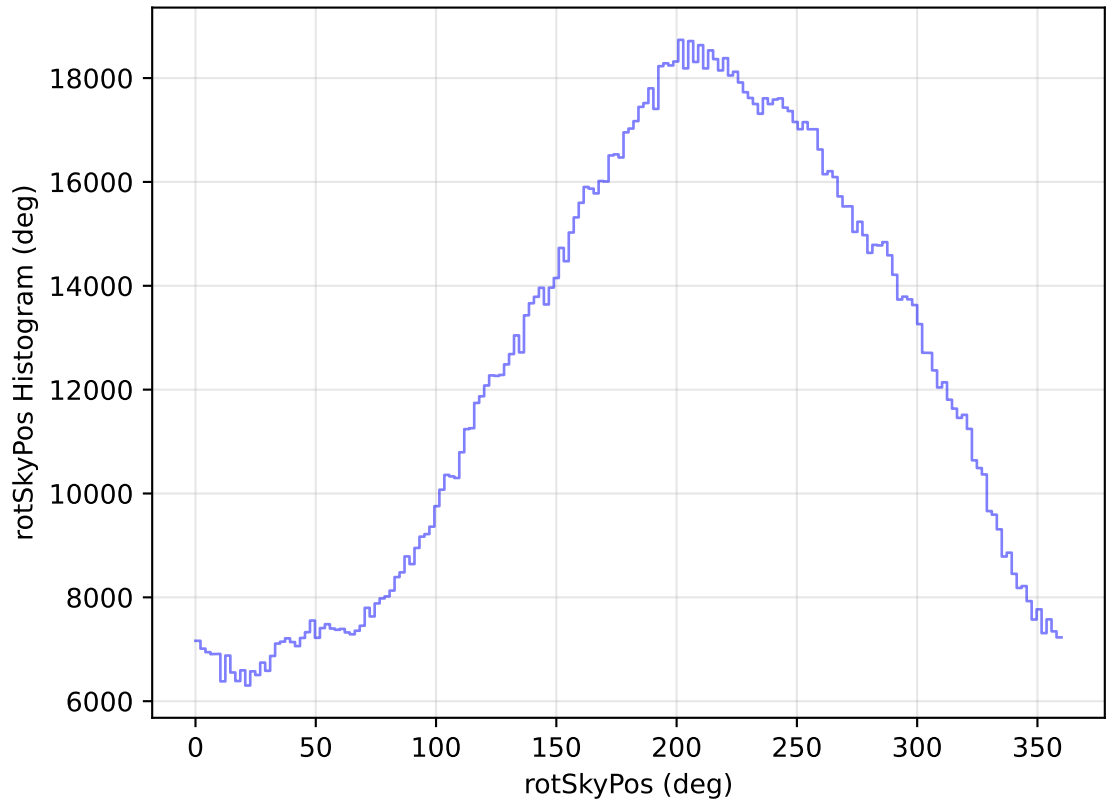
too_elab_heavy_r32_d3_gz_v3.4_10yrs All sky all bands: rotSkyPos Histogram
