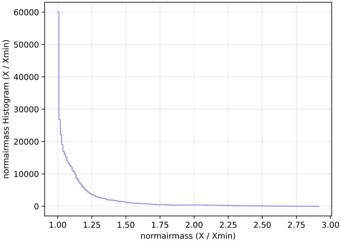
too_elab_heavy_r32_d3_gz_v3.4_10yrs WFD z band: normairmass Histogram
