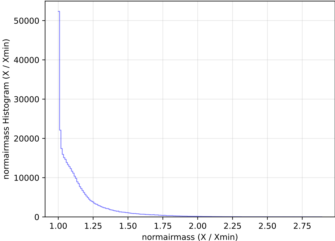
too_elab_heavy_r32_d3_gz_v3.4_10yrs WFD y band: normairmass Histogram
