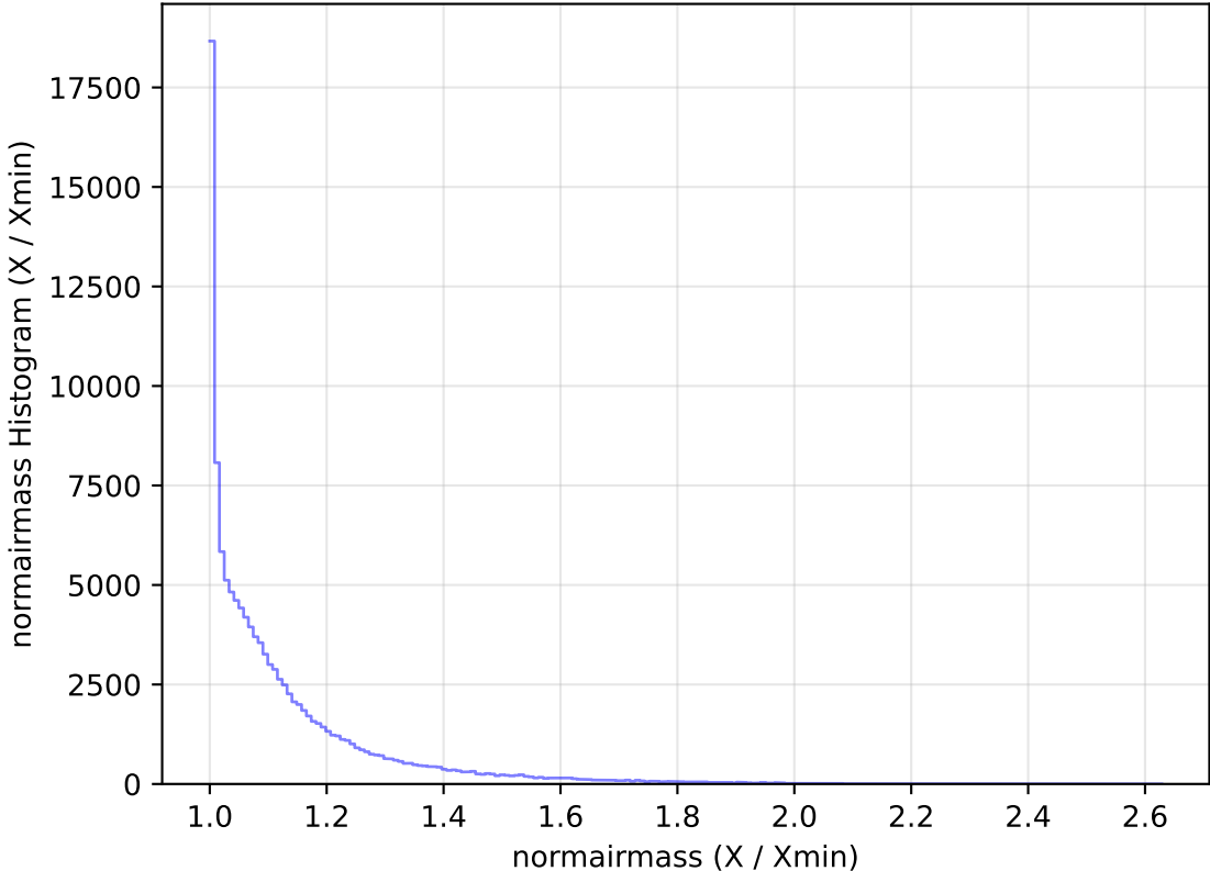
too_elab_heavy_r32_d3_gz_v3.4_10yrs WFD u band: normairmass Histogram
