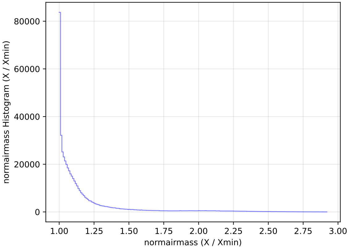
too_elab_heavy_r32_d3_gz_v3.4_10yrs WFD i band: normairmass Histogram
