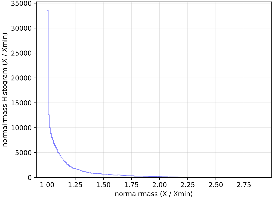
too_elab_heavy_r32_d3_gz_v3.4_10yrs WFD g band: normairmass Histogram
