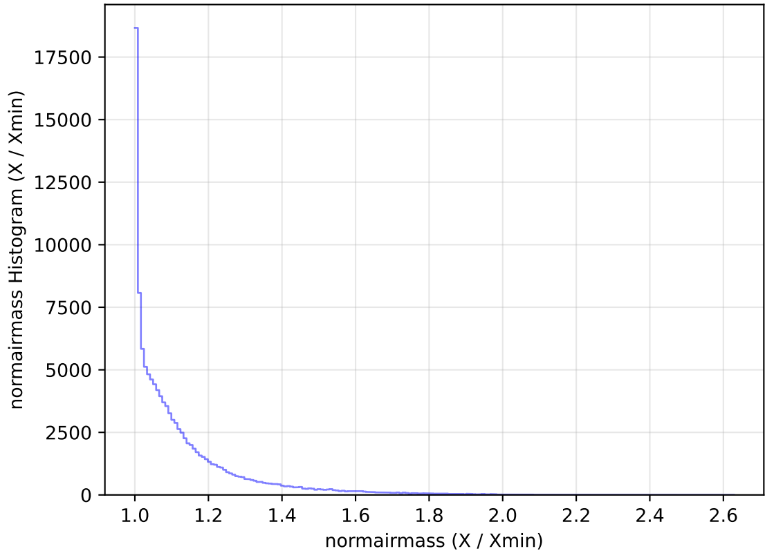
too_elab_heavy_r32_d3_gz_v3.4_10yrs All sky u band: normairmass Histogram
