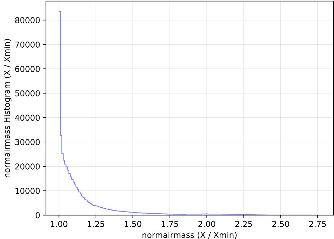
too_elab_heavy_r32_d3_gz_v3.4_10yrs All sky r band: normairmass Histogram
