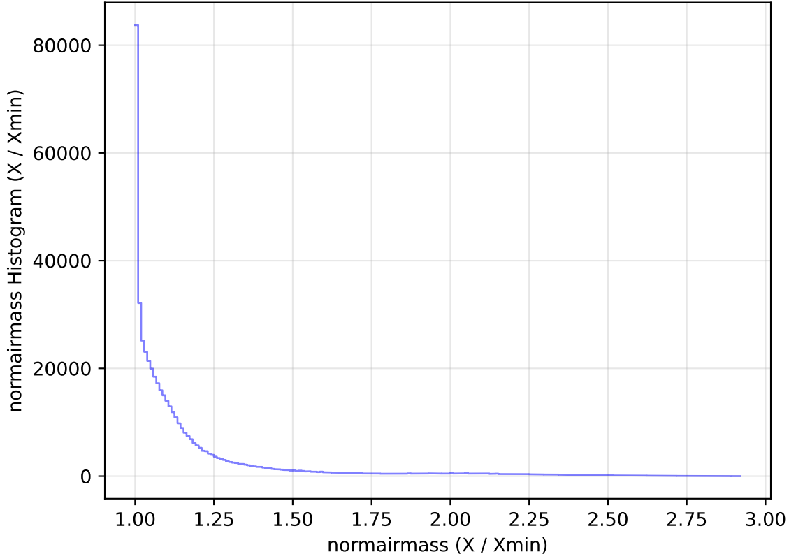
too_elab_heavy_r32_d3_gz_v3.4_10yrs All sky i band: normairmass Histogram
