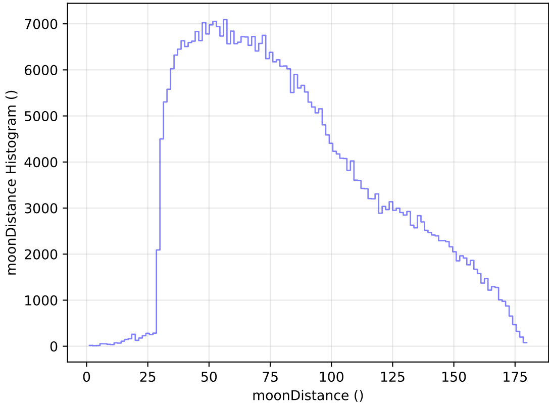
too_elab_heavy_r32_d3_gz_v3.4_10yrs WFD z band: moonDistance Histogram
