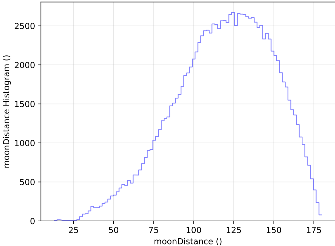
too_elab_heavy_r32_d3_gz_v3.4_10yrs WFD u band: moonDistance Histogram
