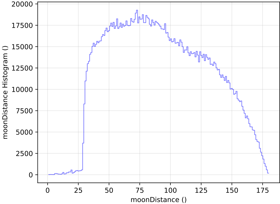
too_elab_heavy_r32_d3_gz_v3.4_10yrs WFD all bands: moonDistance Histogram
