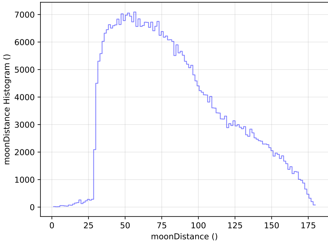
too_elab_heavy_r32_d3_gz_v3.4_10yrs All sky z band: moonDistance Histogram
