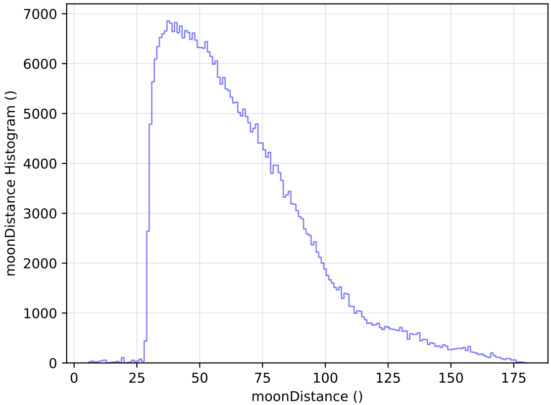
too_elab_heavy_r32_d3_gz_v3.4_10yrs All sky y band: moonDistance Histogram
