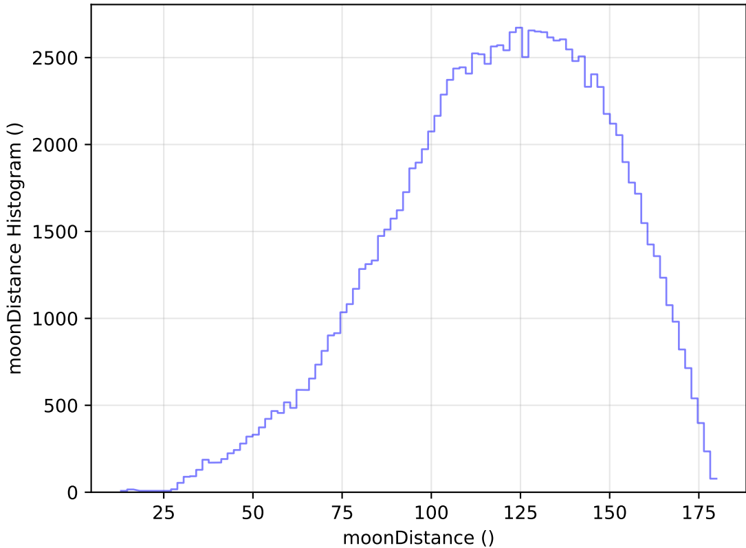
too_elab_heavy_r32_d3_gz_v3.4_10yrs All sky u band: moonDistance Histogram
