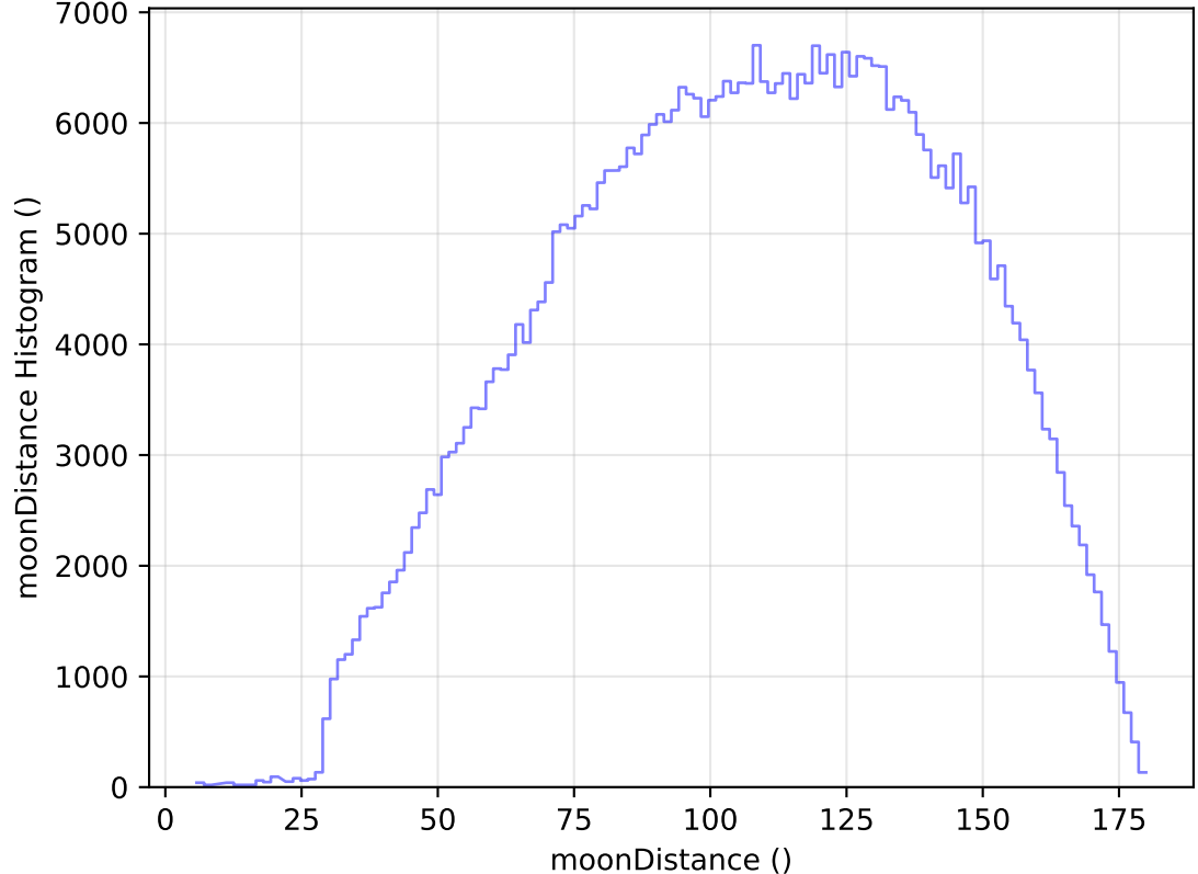
too_elab_heavy_r32_d3_gz_v3.4_10yrs All sky r band: moonDistance Histogram
