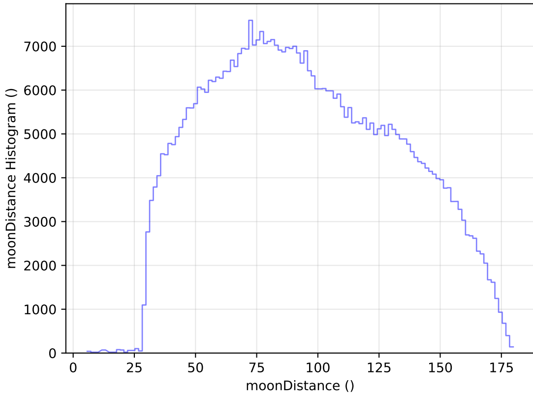
too_elab_heavy_r32_d3_gz_v3.4_10yrs All sky i band: moonDistance Histogram
