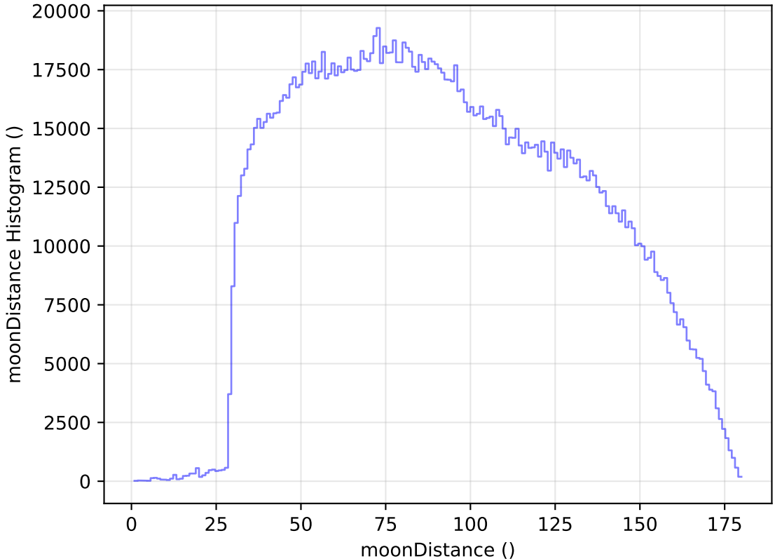
too_elab_heavy_r32_d3_gz_v3.4_10yrs All sky all bands: moonDistance Histogram
