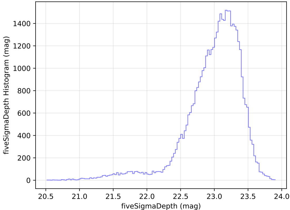
too_elab_heavy_r32_d3_gz_v3.4_10yrs Yr 1 z band: fiveSigmaDepth Histogram
