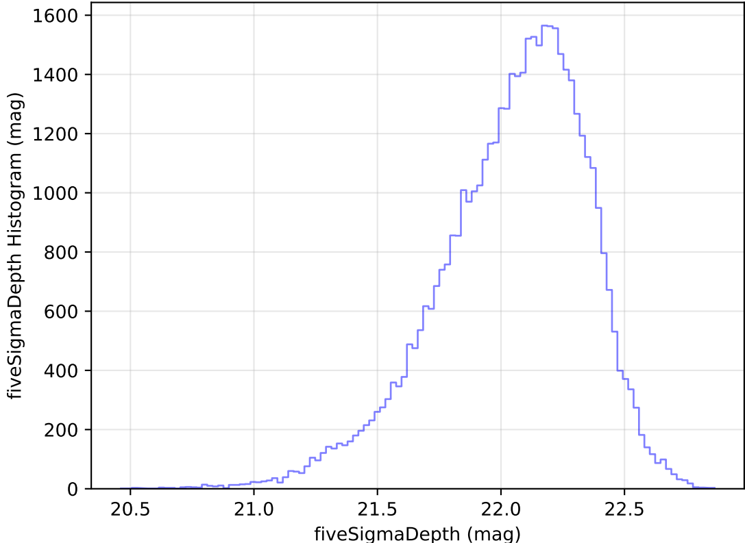
too_elab_heavy_r32_d3_gz_v3.4_10yrs Yr 1 y band: fiveSigmaDepth Histogram
