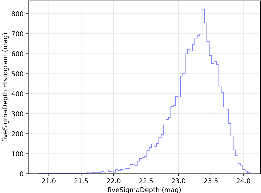
too_elab_heavy_r32_d3_gz_v3.4_10yrs Yr 1 u band: fiveSigmaDepth Histogram
