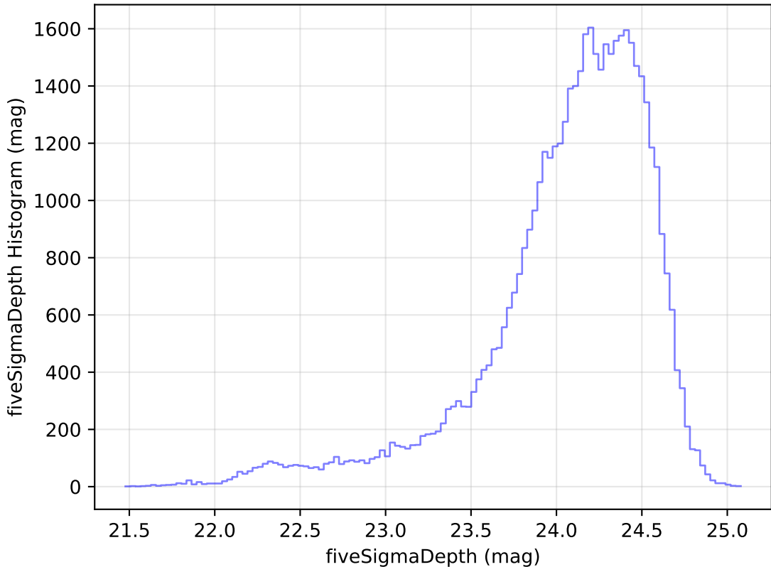
too_elab_heavy_r32_d3_gz_v3.4_10yrs Yr 1 r band: fiveSigmaDepth Histogram
