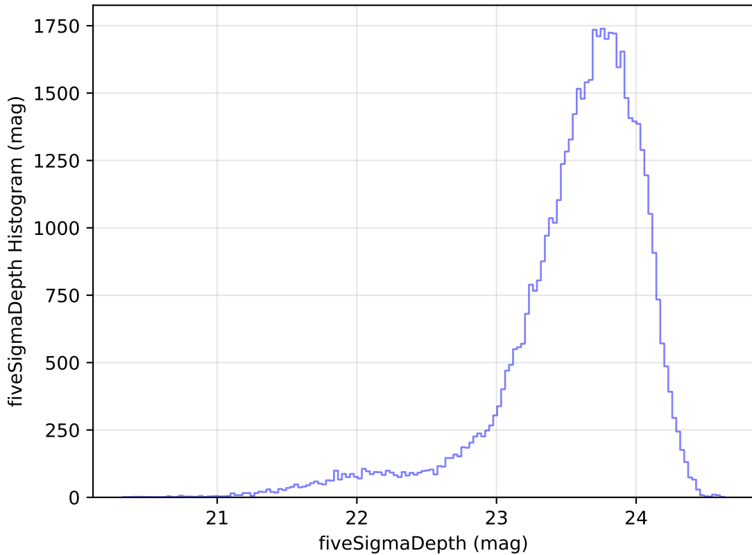
too_elab_heavy_r32_d3_gz_v3.4_10yrs Yr 1 i band: fiveSigmaDepth Histogram
