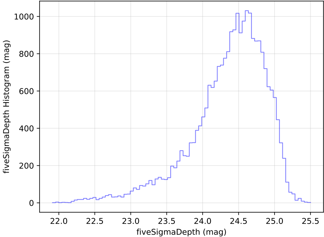
too_elab_heavy_r32_d3_gz_v3.4_10yrs Yr 1 g band: fiveSigmaDepth Histogram
