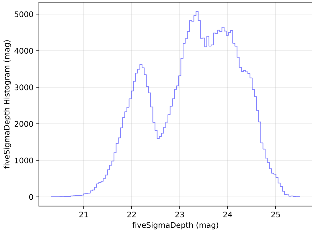
too_elab_heavy_r32_d3_gz_v3.4_10yrs Yr 1 all bands: fiveSigmaDepth Histogram
