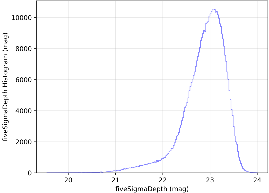
too_elab_heavy_r32_d3_gz_v3.4_10yrs WFD z band: fiveSigmaDepth Histogram
