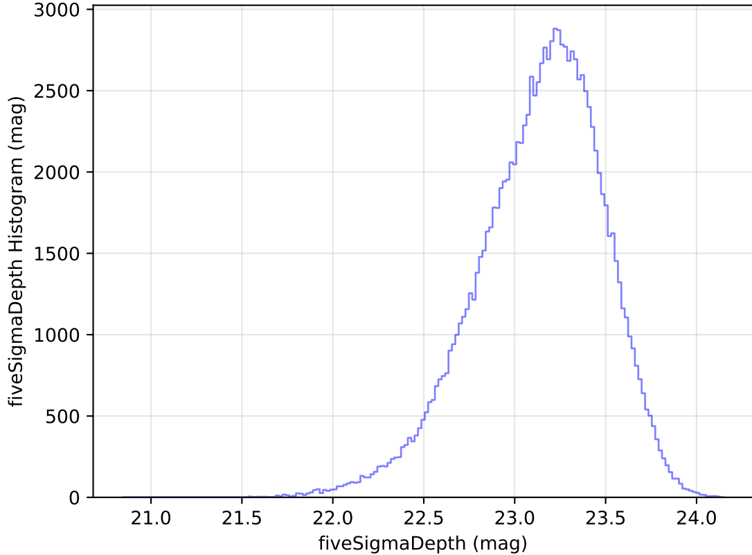
too_elab_heavy_r32_d3_gz_v3.4_10yrs WFD u band: fiveSigmaDepth Histogram
