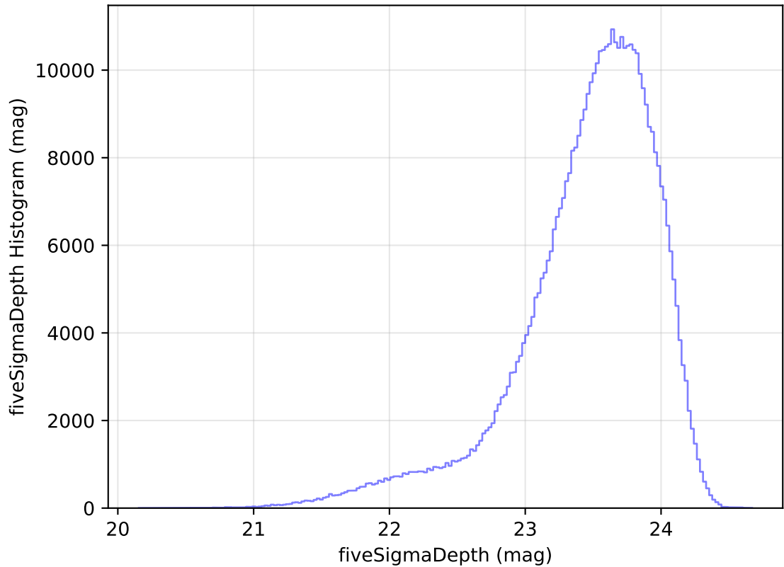
too_elab_heavy_r32_d3_gz_v3.4_10yrs WFD i band: fiveSigmaDepth Histogram
