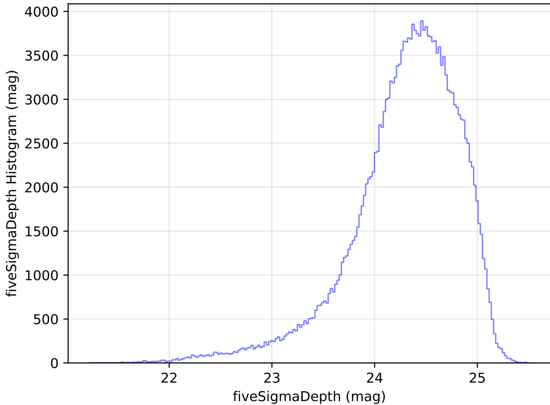
too_elab_heavy_r32_d3_gz_v3.4_10yrs WFD g band: fiveSigmaDepth Histogram
