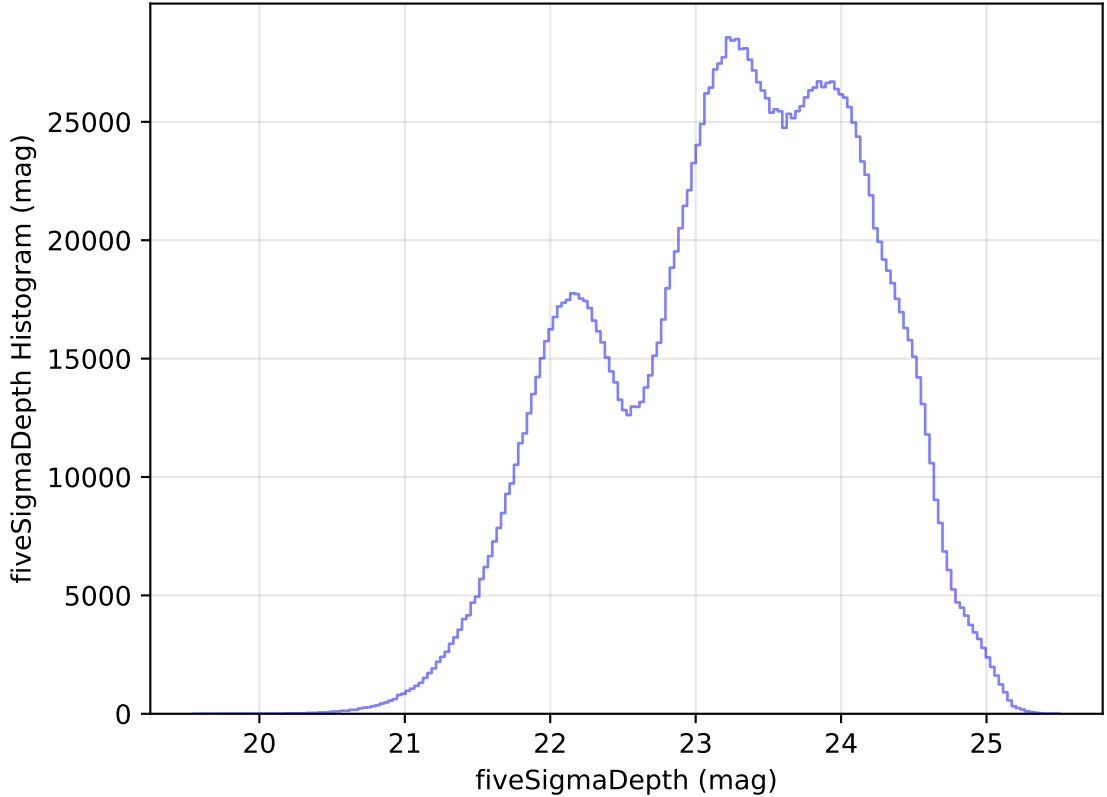
too_elab_heavy_r32_d3_gz_v3.4_10yrs WFD all bands: fiveSigmaDepth Histogram
