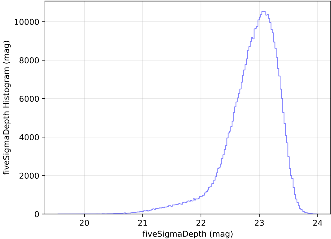
too_elab_heavy_r32_d3_gz_v3.4_10yrs All sky z band: fiveSigmaDepth Histogram
