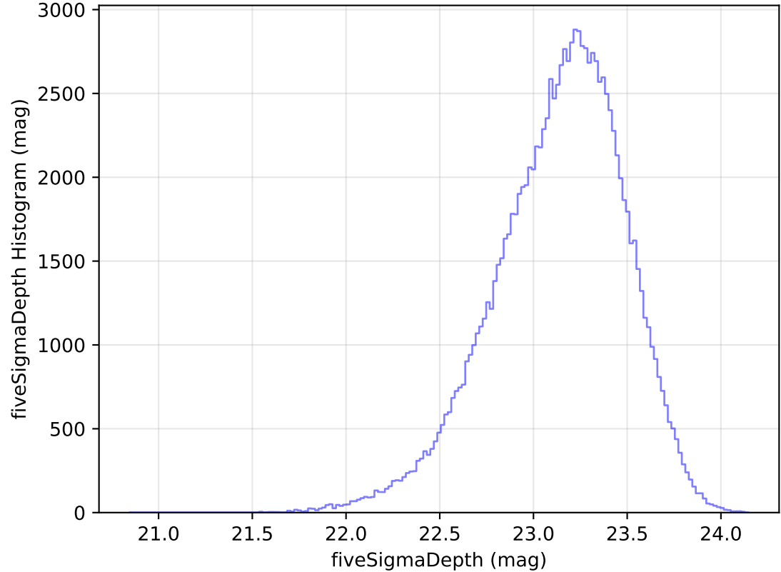
too_elab_heavy_r32_d3_gz_v3.4_10yrs All sky u band: fiveSigmaDepth Histogram
