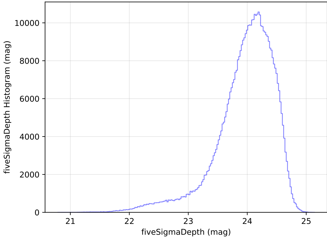
too_elab_heavy_r32_d3_gz_v3.4_10yrs All sky r band: fiveSigmaDepth Histogram
