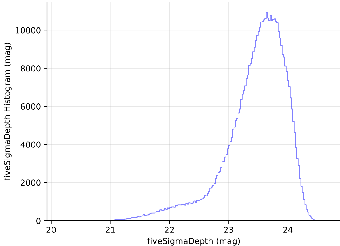
too_elab_heavy_r32_d3_gz_v3.4_10yrs All sky i band: fiveSigmaDepth Histogram
